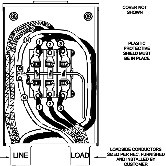
UNDERGROUND SERVICE CONDUCTORS SIZED PER NEC, FURNISHED AND INSTALLED BY CUSTOMER
